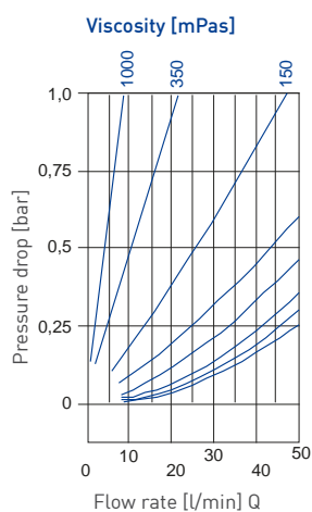
Typical pressure drop V05
