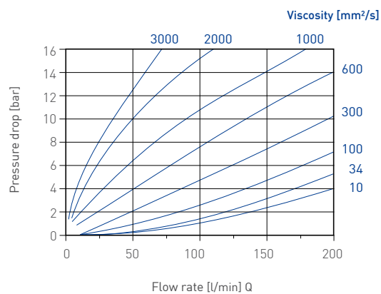
Typical pressure drop VZ5AL
